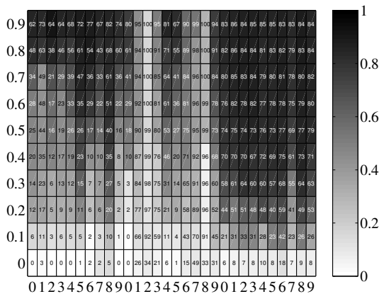
Fig. 6: All words used for keyword extraction. First (second and third) 0 to 9 columns: AHA, General and Radiology data-bases, respectively. Numbers on the vertical axis: Threshold values. Numbers in boxes: number of representative key-words chosen from all words. Gray scale: OR qualities of clustering at different thresholds.
